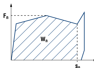
Statisches DEFORM plus® - Diagramm Static DEFORM plus® - diagram
